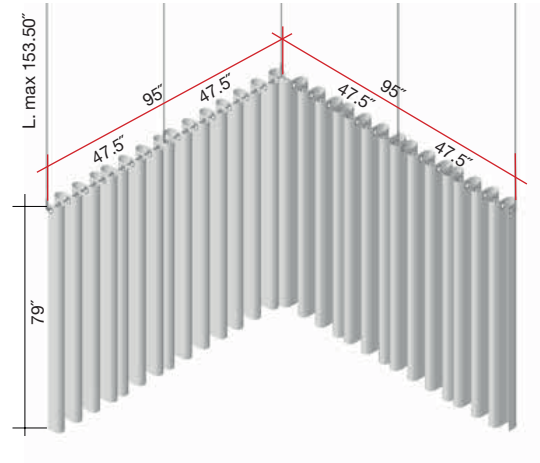
ITEM# 40041017: 4 ft SUPPORT ROD (X4) ITEM# 40041024: END SUPPORTS (X2) ITEM# 40041026: CORNER SUPPORTS (X1) ITEM# 40041025: CENTRAL SUPPORTS (X2) TEXTILE PANEL: (X8)
