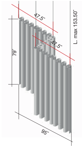
ITEM# 40041017: 4 ft SUPPORT ROD (X2) ITEM# 40041016: 2 ft SUPPORT ROD (X1) ITEM# 40041024: END SUPPORTS (X2) ITEM# 40041026: CORNER SUPPORTS (X2) ITEM# 40041025: CENTRAL SUPPORTS (X2) TEXTILE PANEL: (X5)
