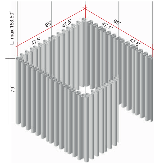
ITEM# 40041017: 4 ft SUPPORT ROD (X7) ITEM# 40041024: END SUPPORTS (X2) ITEM# 40041026: CORNER SUPPORTS (X3) ITEM# 40041025: CENTRAL SUPPORTS (X3) TEXTILE PANEL: (X14)
